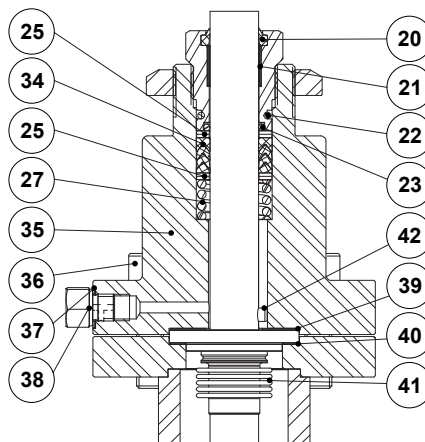
Bellows sealing (BV1)
