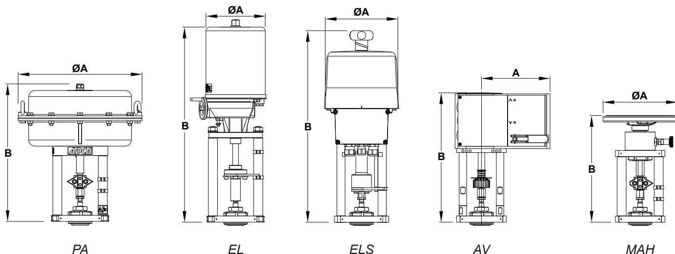
DIMENSIONS – PA SERIES PNEUMATIC ACTUATORS (mm)
