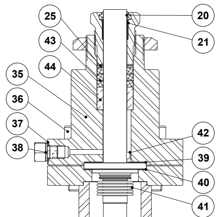
Bellows sealing (BG1)
