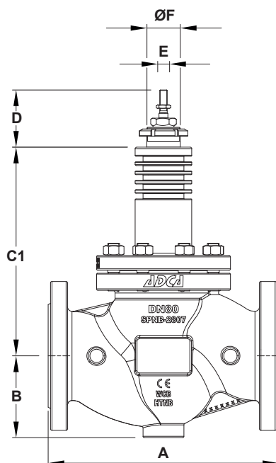
Valve with extended bonnet
