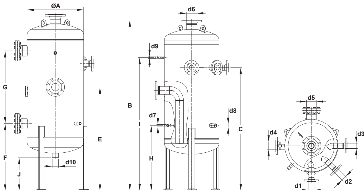
DIMENSIONS (mm) *
